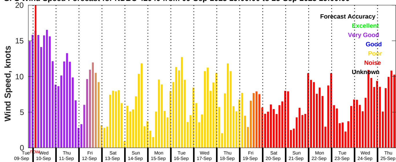
GFS Wind Speed Forecast for NDBC 42040 from 09-Sep-2025 19:00:00 to 25-Sep-2025 19:00:00
