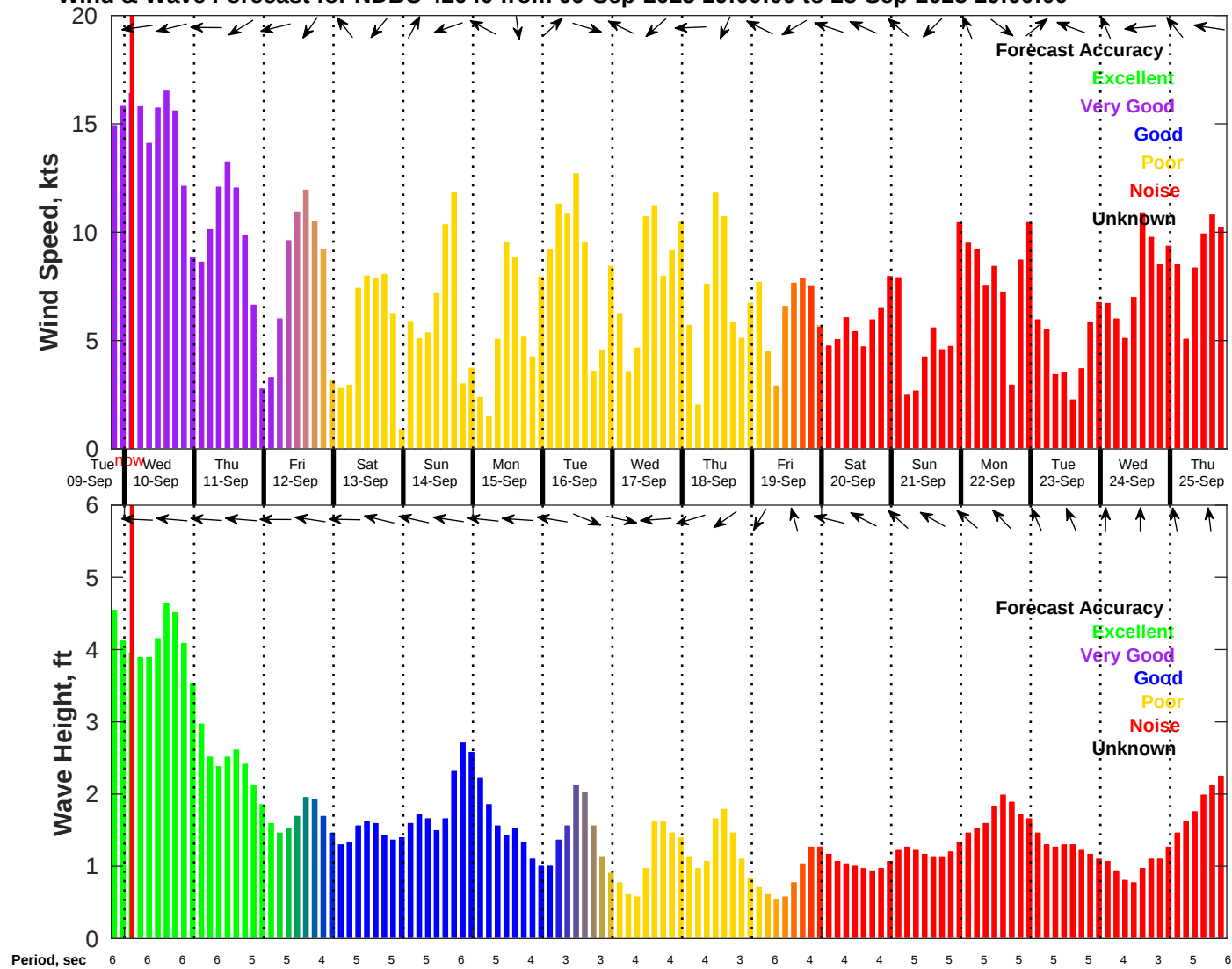
Wind & Wave Forecast for NDBC 42040 from 09-Sep-2025 19:00:00 to 25-Sep-2025 19:00:00
