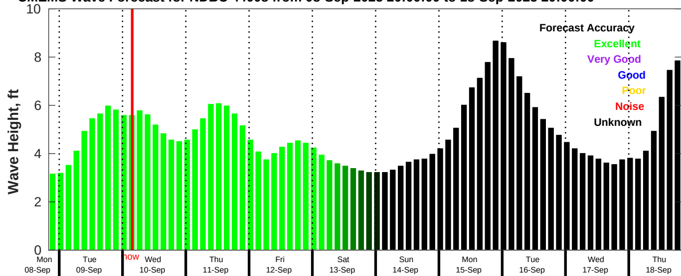
CMEMS Wave Forecast for NDBC 44008 from 08-Sep-2025 20:00:00 to 18-Sep-2025 20:00:00
