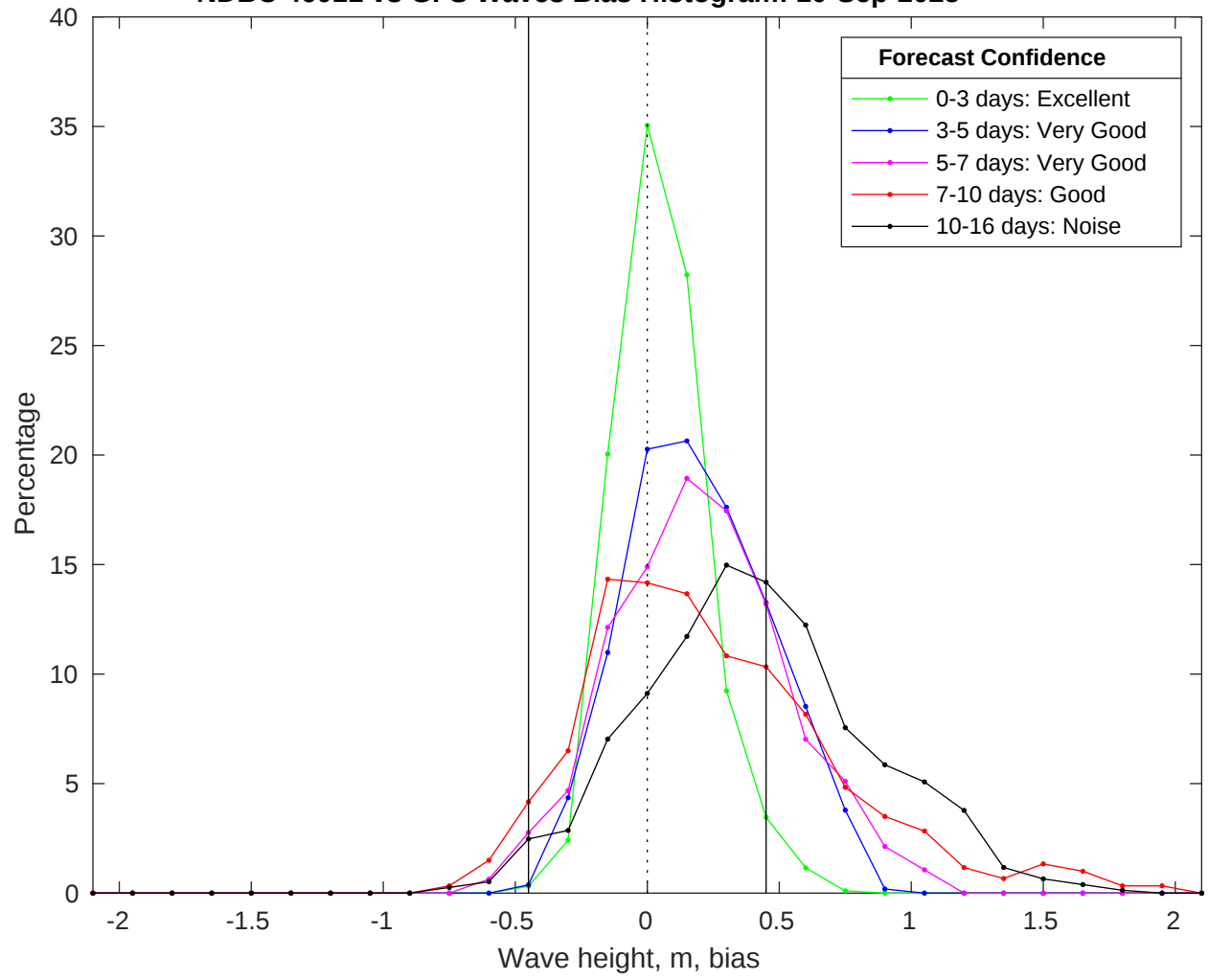
NDBC 46011 vs GFS Waves Bias Histogram: 10-Sep-2025
