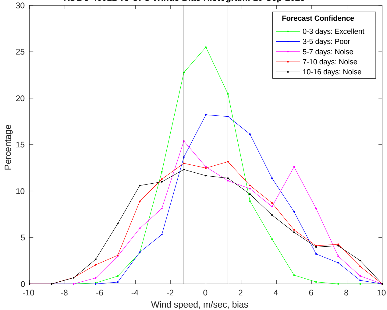
NDBC 46011 vs GFS Winds Bias Histogram: 10-Sep-2025
