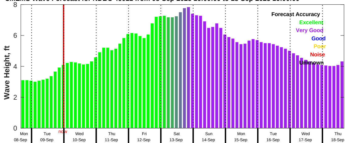
CMEMS Wave Forecast for NDBC 46011 from 08-Sep-2025 16:00:00 to 18-Sep-2025 16:00:00
