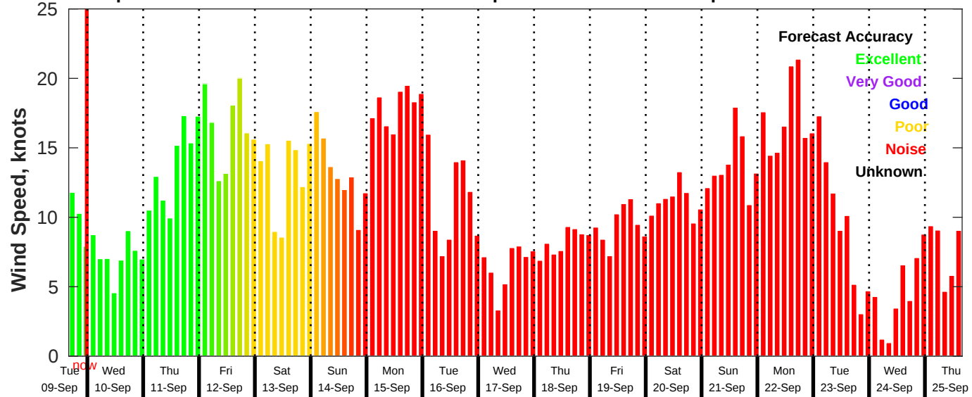
GFS Wind Speed Forecast for NDBC 46011 from 09-Sep-2025 16:00:00 to 25-Sep-2025 16:00:00
