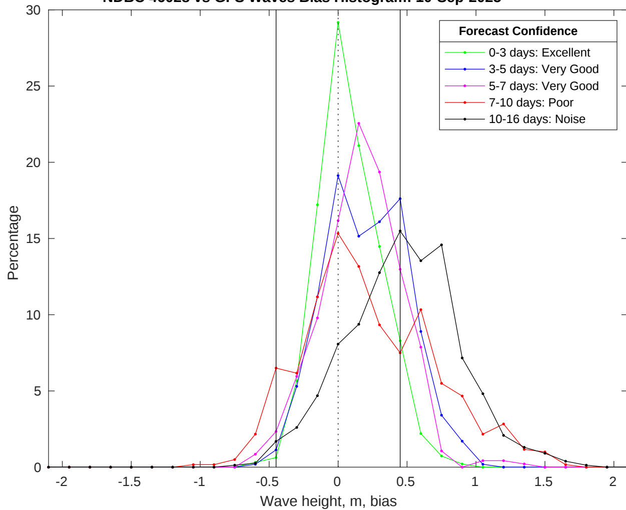
NDBC 46028 vs GFS Waves Bias Histogram: 10-Sep-2025
