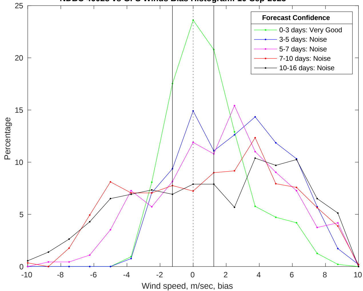
NDBC 46028 vs GFS Winds Bias Histogram: 10-Sep-2025
