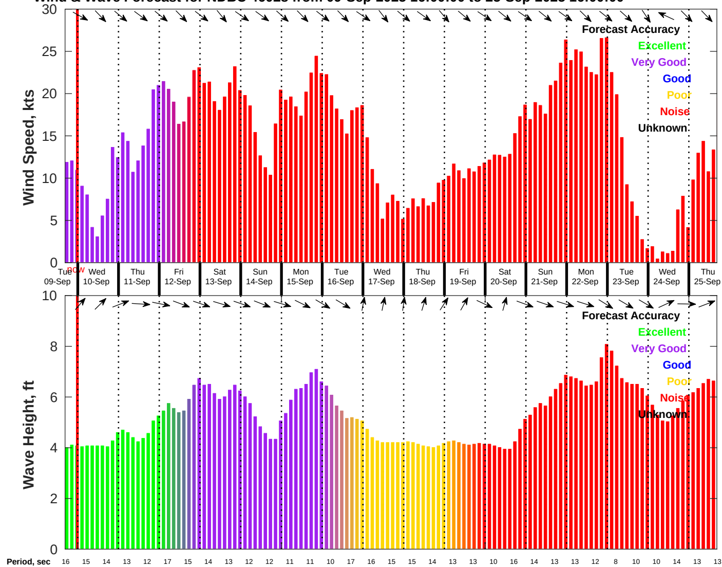
Wind & Wave Forecast for NDBC 46028 from 09-Sep-2025 16:00:00 to 25-Sep-2025 16:00:00
