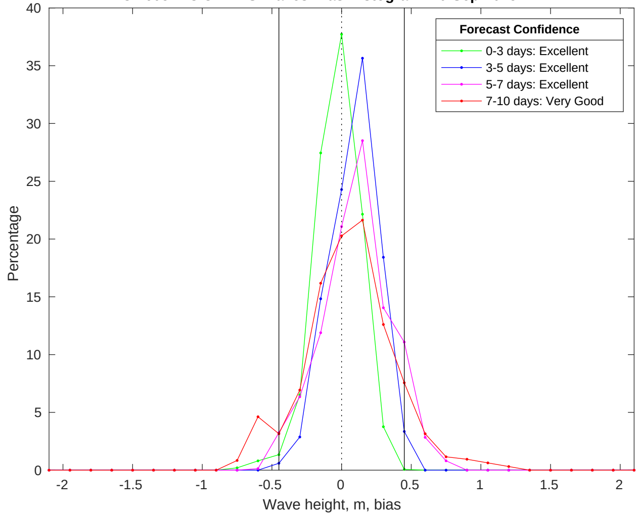
NDBC 46054 vs CMEMS Waves Bias Histogram: 10-Sep-2025
