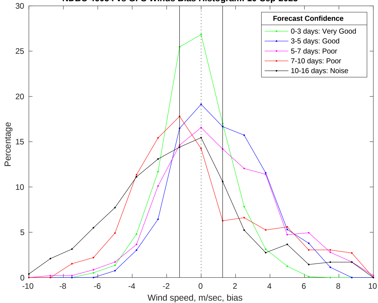
NDBC 46054 vs GFS Winds Bias Histogram: 10-Sep-2025
