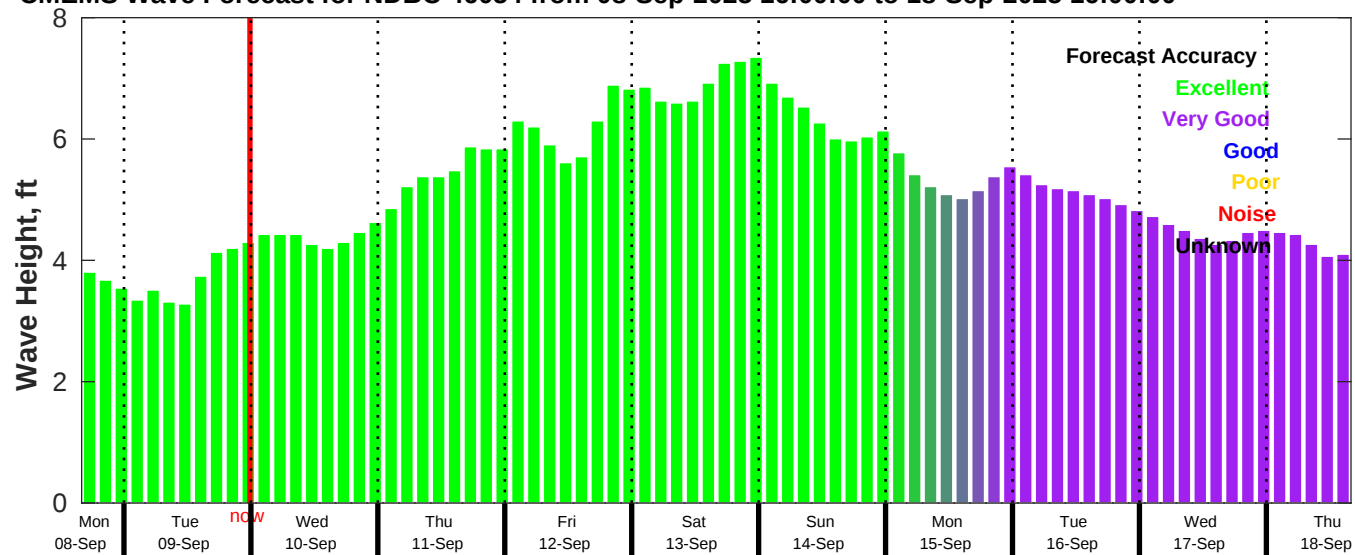
CMEMS Wave Forecast for NDBC 46054 from 08-Sep-2025 16:00:00 to 18-Sep-2025 16:00:00
