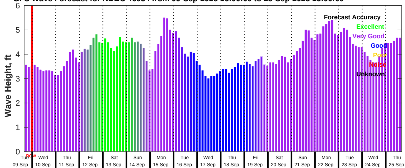
GFS Wave Forecast for NDBC 46054 from 09-Sep-2025 16:00:00 to 25-Sep-2025 16:00:00
