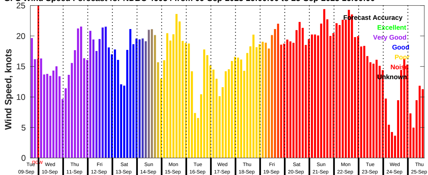
GFS Wind Speed Forecast for NDBC 46054 from 09-Sep-2025 16:00:00 to 25-Sep-2025 16:00:00
