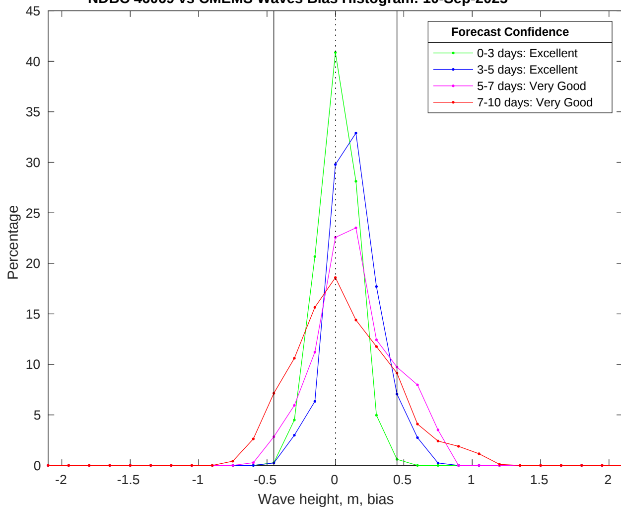
NDBC 46069 vs CMEMS Waves Bias Histogram: 10-Sep-2025
