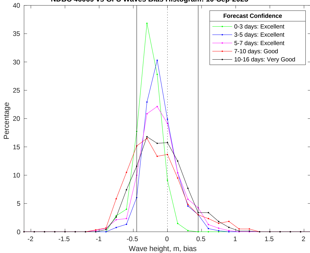
NDBC 46069 vs GFS Waves Bias Histogram: 10-Sep-2025
