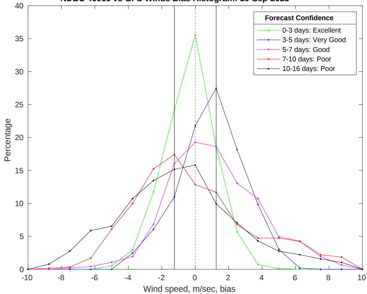
NDBC 46069 vs GFS Winds Bias Histogram: 10-Sep-2025
