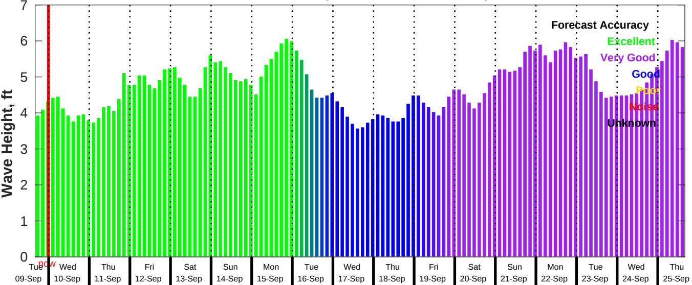
GFS Wave Forecast for NDBC 46069 from 09-Sep-2025 16:00:00 to 25-Sep-2025 16:00:00
