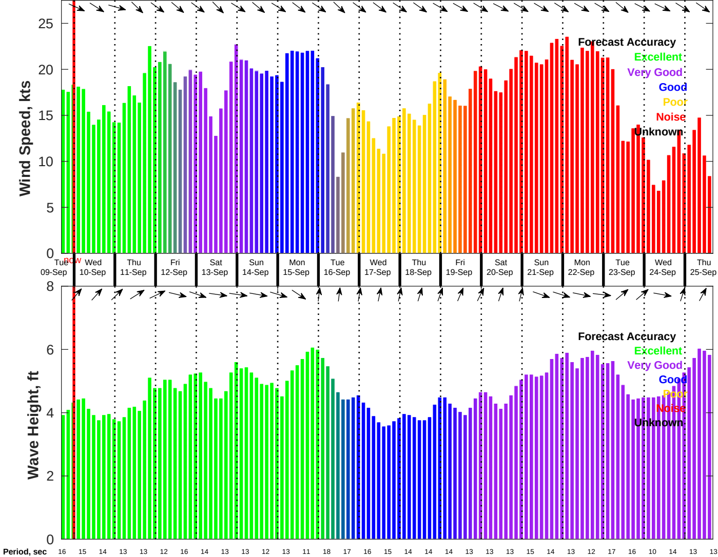
Wind & Wave Forecast for NDBC 46069 from 09-Sep-2025 16:00:00 to 25-Sep-2025 16:00:00
