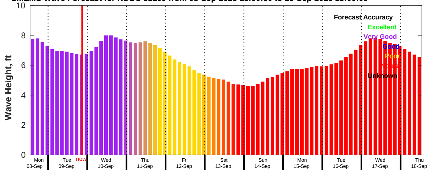
CMEMS Wave Forecast for NDBC 51209 from 08-Sep-2025 13:00:00 to 18-Sep-2025 13:00:00
