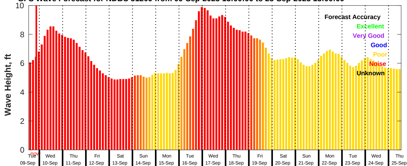
GFS Wave Forecast for NDBC 51209 from 09-Sep-2025 13:00:00 to 25-Sep-2025 13:00:00
