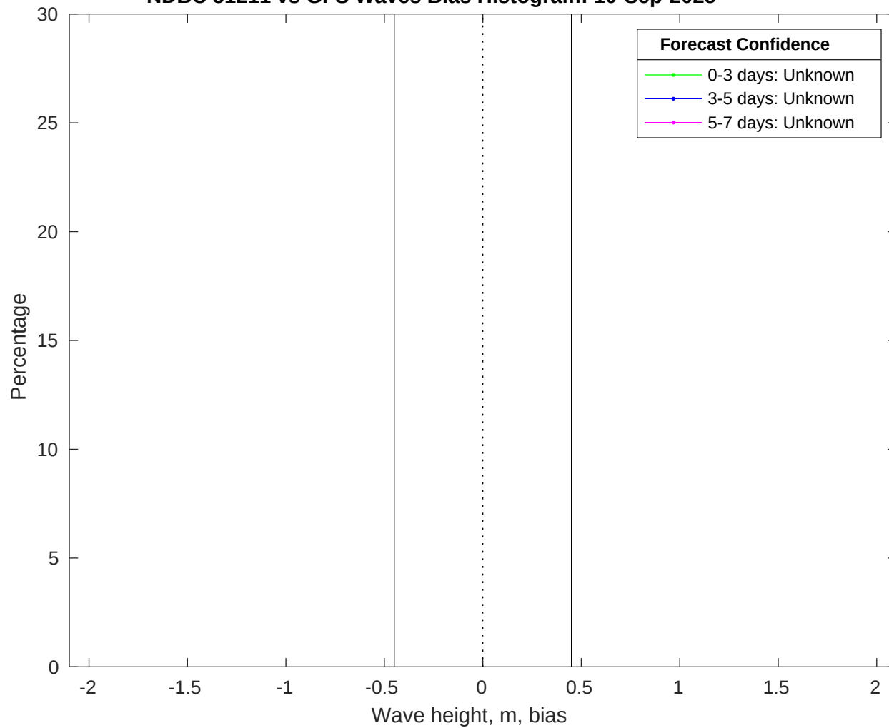
NDBC 51211 vs GFS Waves Bias Histogram: 10-Sep-2025
