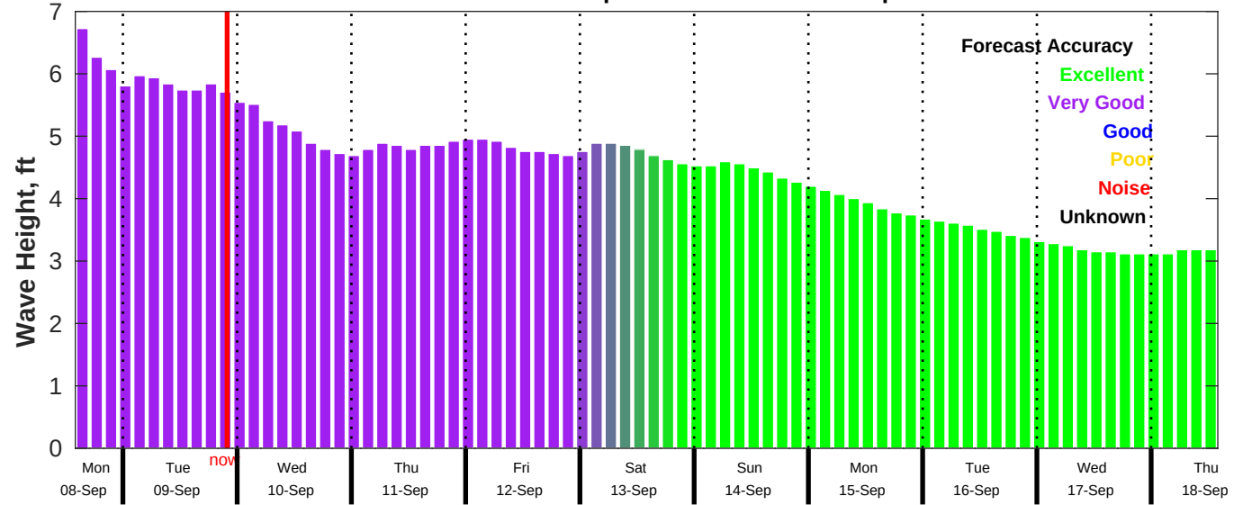
CMEMS Wave Forecast for NDBC 51211 from 08-Sep-2025 14:00:00 to 18-Sep-2025 14:00:00
