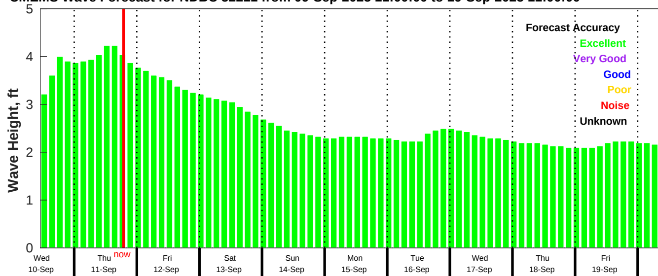
CMEMS Wave Forecast for NDBC 52211 from 09-Sep-2025 11:00:00 to 19-Sep-2025 11:00:00
