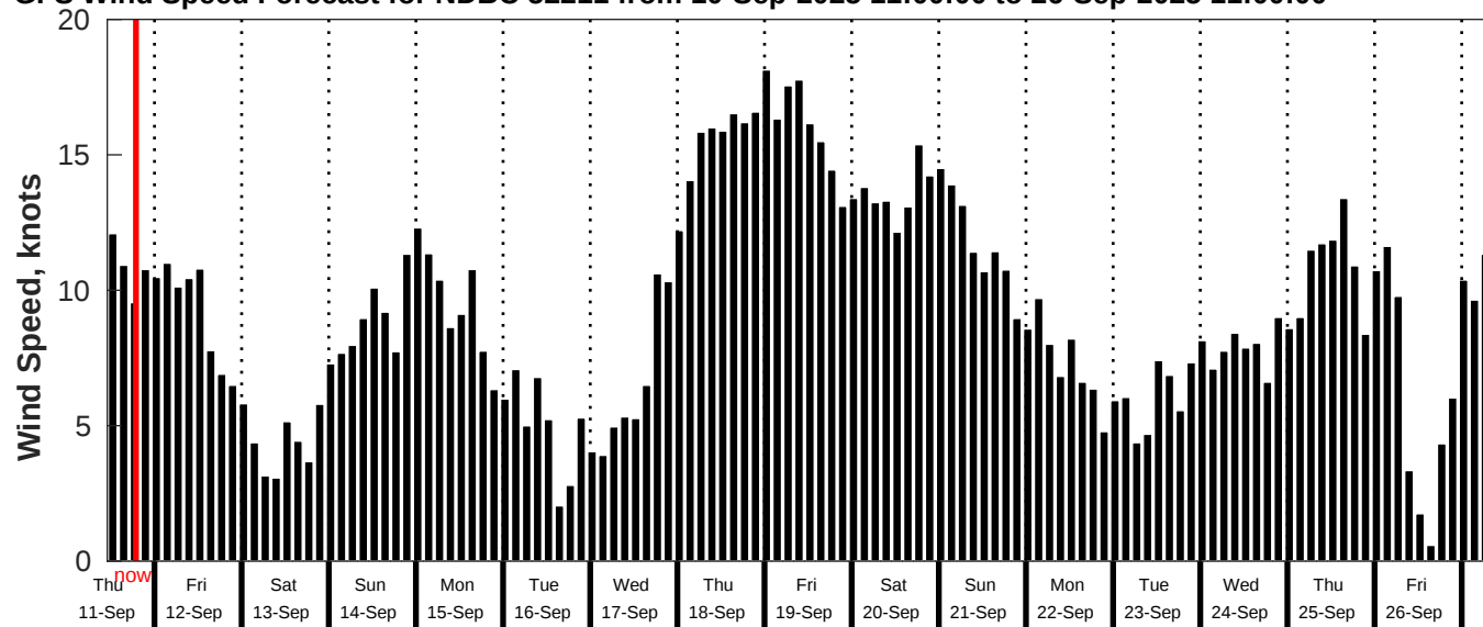
GFS Wind Speed Forecast for NDBC 52211 from 10-Sep-2025 11:00:00 to 26-Sep-2025 11:00:00
