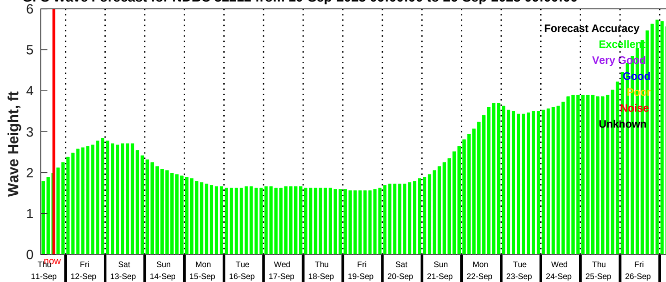
GFS Wave Forecast for NDBC 52212 from 10-Sep-2025 09:00:00 to 26-Sep-2025 09:00:00
