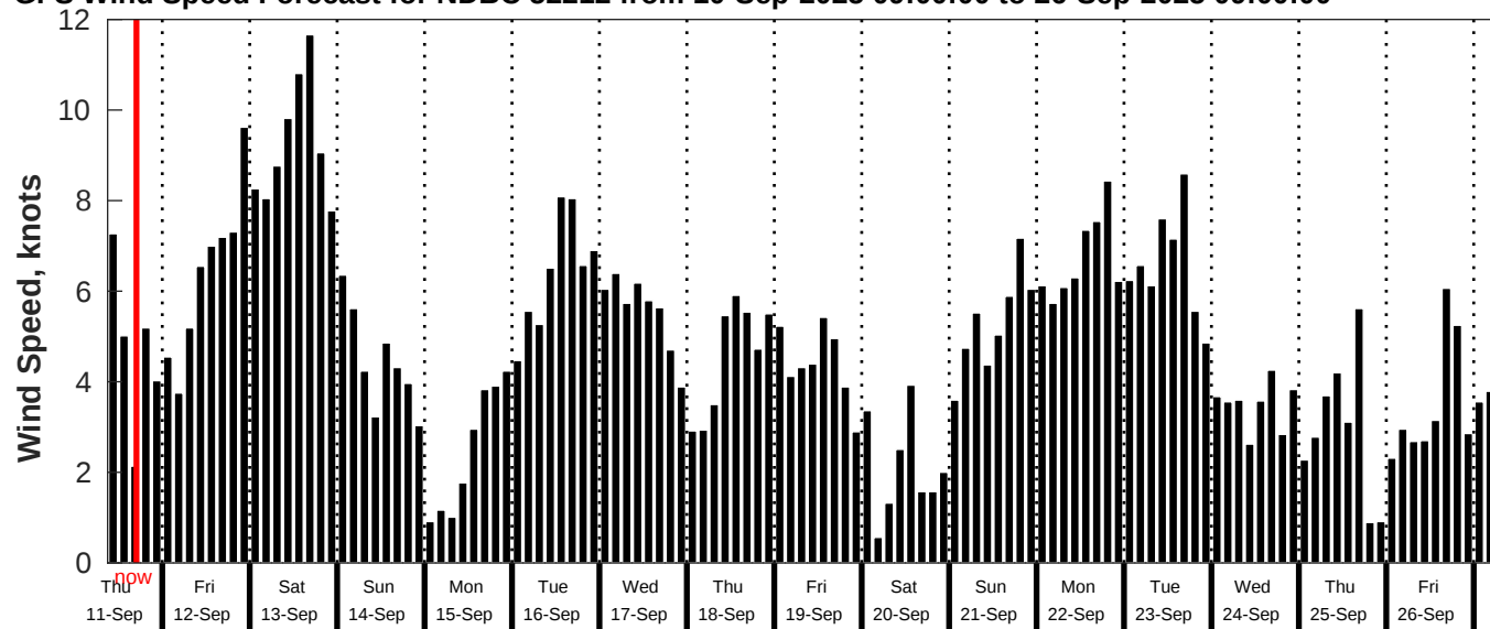
GFS Wind Speed Forecast for NDBC 52212 from 10-Sep-2025 09:00:00 to 26-Sep-2025 09:00:00
