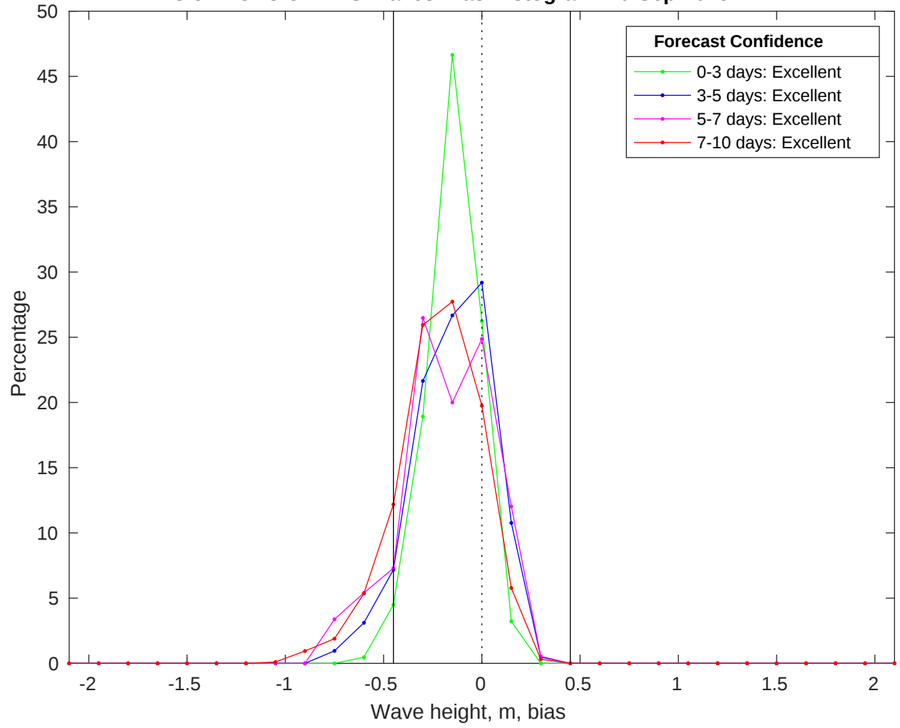
NDBC 52213 vs CMEMS Waves Bias Histogram: 10-Sep-2025
