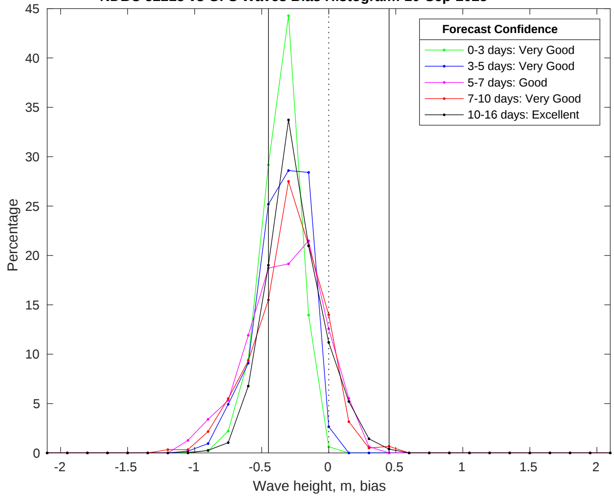
NDBC 52213 vs GFS Waves Bias Histogram: 10-Sep-2025
