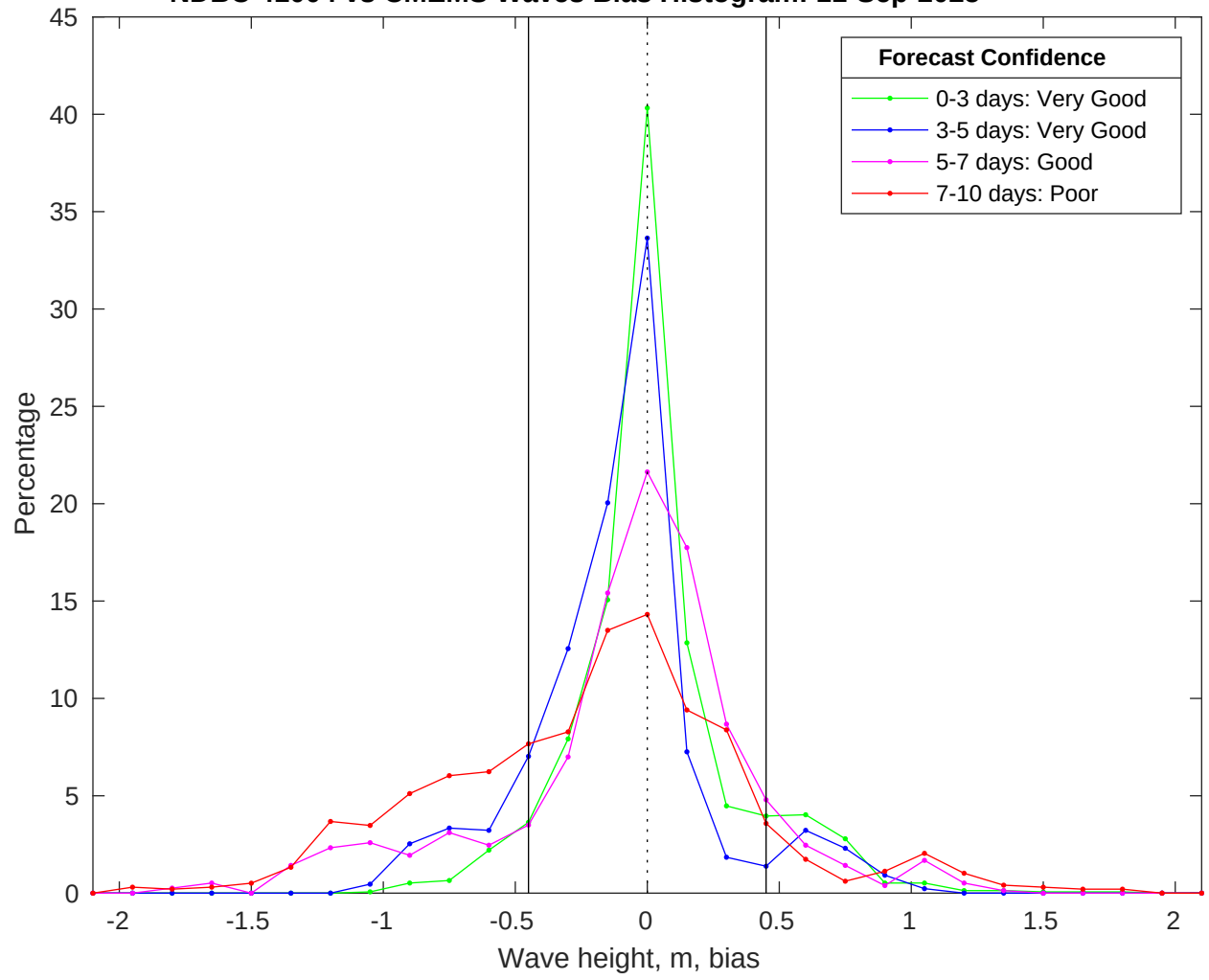
NDBC 41004 vs CMEMS Waves Bias Histogram: 11-Sep-2025
