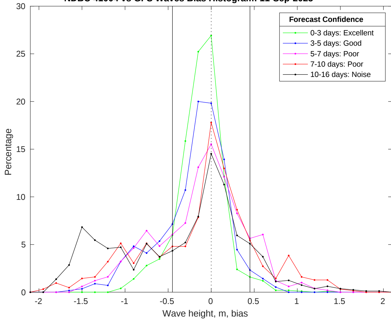
NDBC 41004 vs GFS Waves Bias Histogram: 11-Sep-2025
