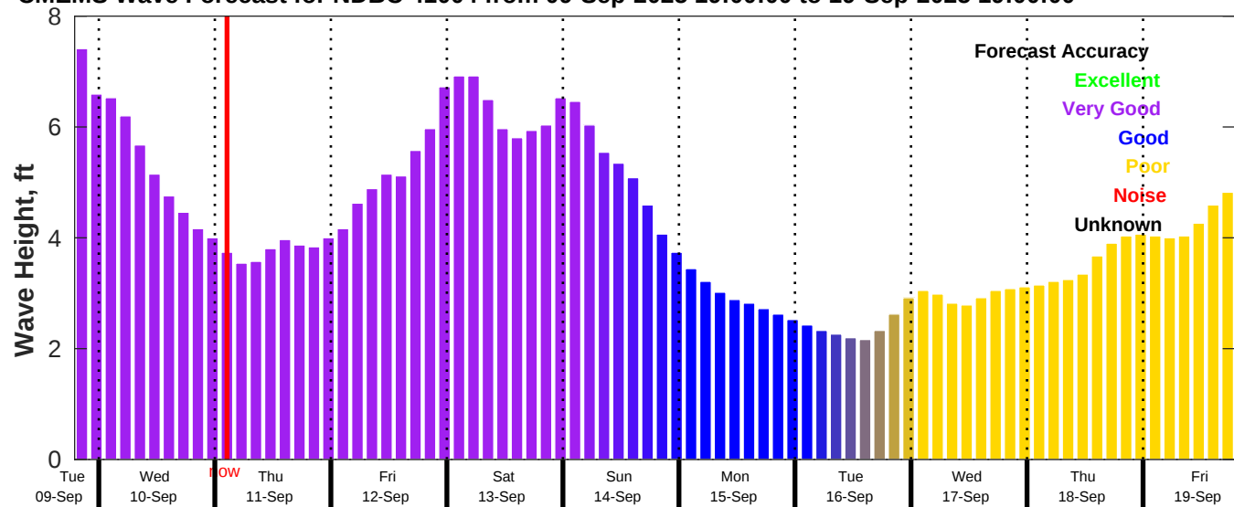
CMEMS Wave Forecast for NDBC 41004 from 09-Sep-2025 19:00:00 to 19-Sep-2025 19:00:00
