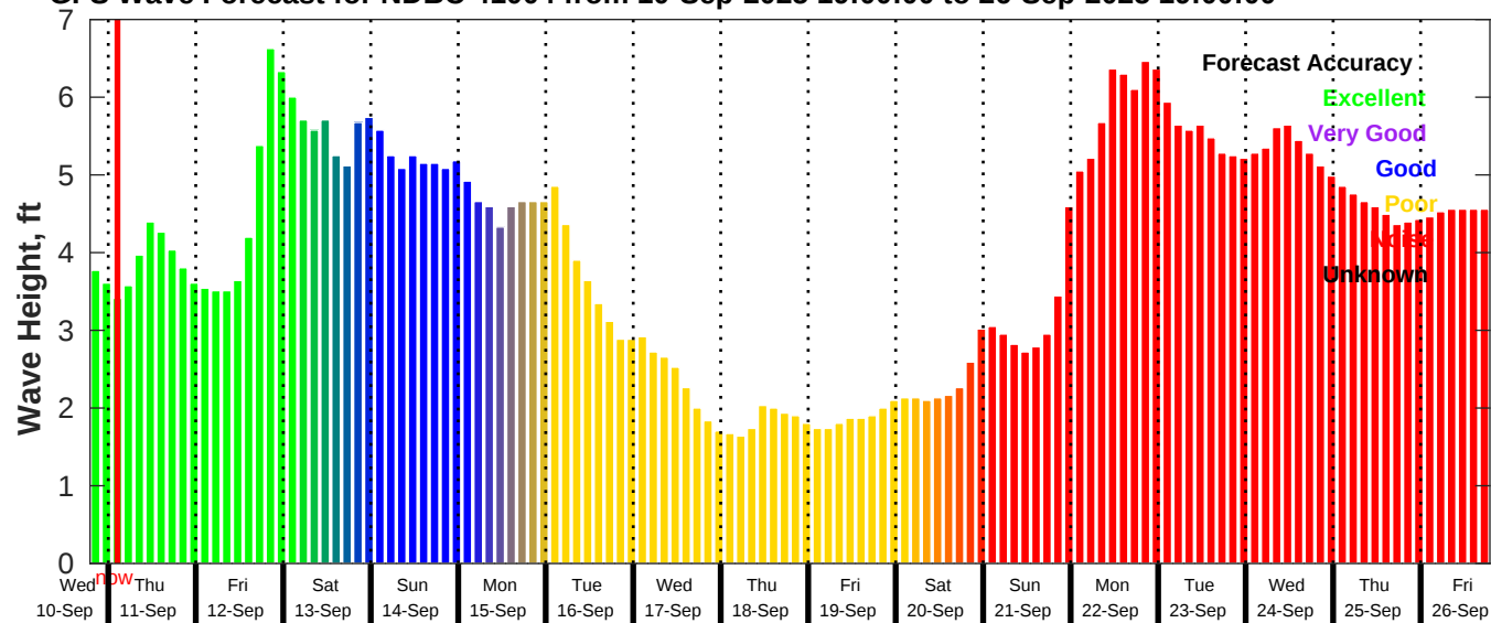
GFS Wave Forecast for NDBC 41004 from 10-Sep-2025 19:00:00 to 26-Sep-2025 19:00:00
