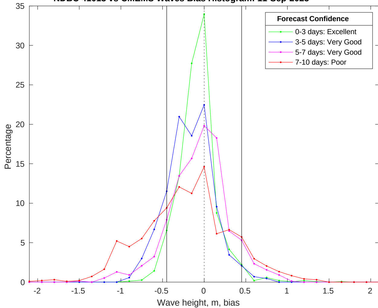
NDBC 41013 vs CMEMS Waves Bias Histogram: 11-Sep-2025
