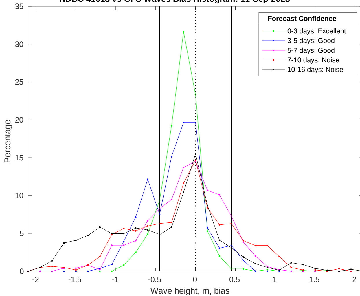
NDBC 41013 vs GFS Waves Bias Histogram: 11-Sep-2025
