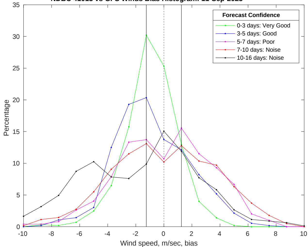
NDBC 41013 vs GFS Winds Bias Histogram: 11-Sep-2025
