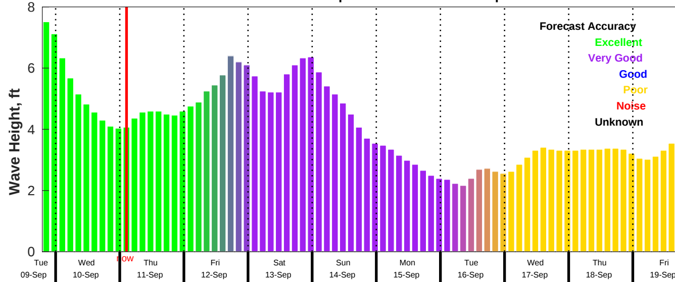
CMEMS Wave Forecast for NDBC 41013 from 09-Sep-2025 19:00:00 to 19-Sep-2025 19:00:00
