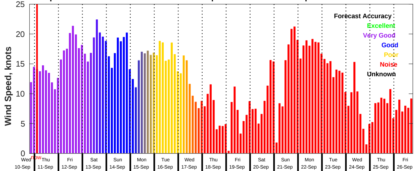
GFS Wind Speed Forecast for NDBC 41013 from 10-Sep-2025 19:00:00 to 26-Sep-2025 19:00:00
