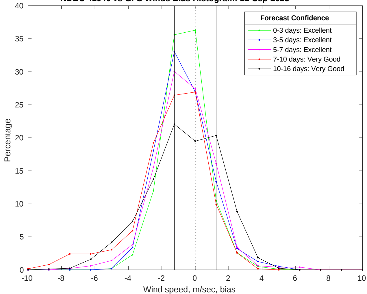
NDBC 41040 vs GFS Winds Bias Histogram: 11-Sep-2025
