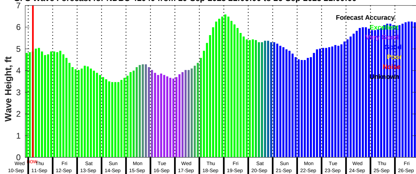
GFS Wave Forecast for NDBC 41040 from 10-Sep-2025 21:00:00 to 26-Sep-2025 21:00:00
