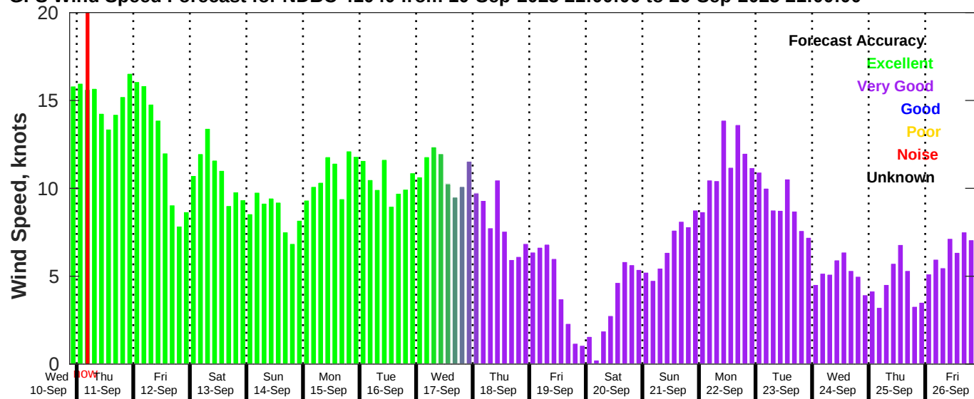
GFS Wind Speed Forecast for NDBC 41040 from 10-Sep-2025 21:00:00 to 26-Sep-2025 21:00:00
