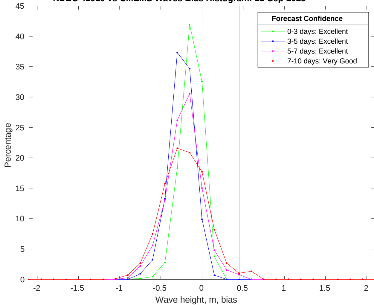
NDBC 42019 vs CMEMS Waves Bias Histogram: 11-Sep-2025
