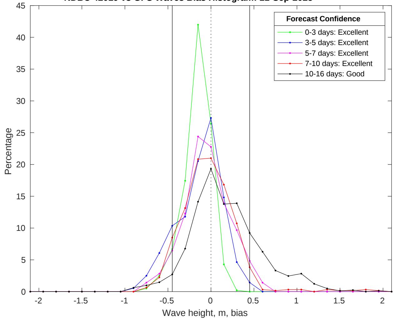
NDBC 42019 vs GFS Waves Bias Histogram: 11-Sep-2025
