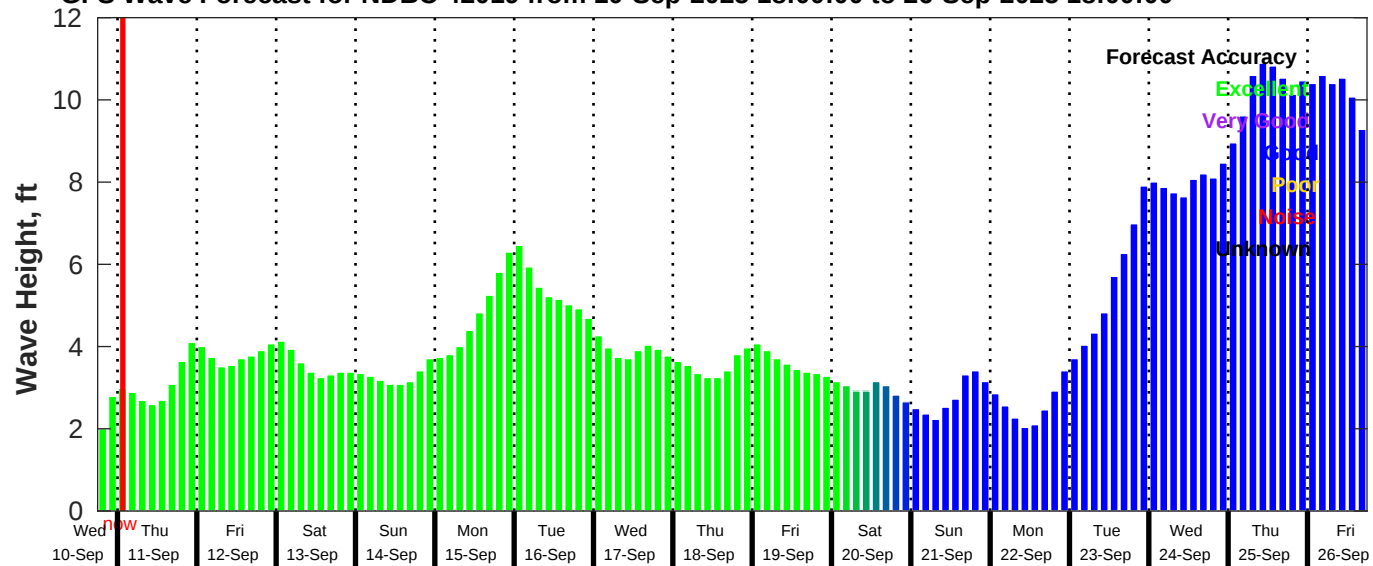
GFS Wave Forecast for NDBC 42019 from 10-Sep-2025 18:00:00 to 26-Sep-2025 18:00:00
