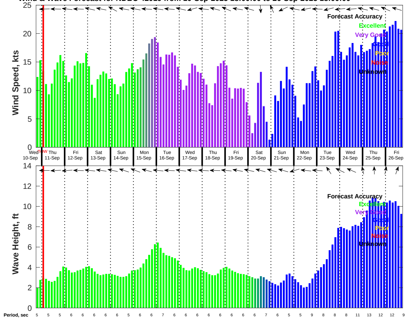
Wind & Wave Forecast for NDBC 42019 from 10-Sep-2025 18:00:00 to 26-Sep-2025 18:00:00
