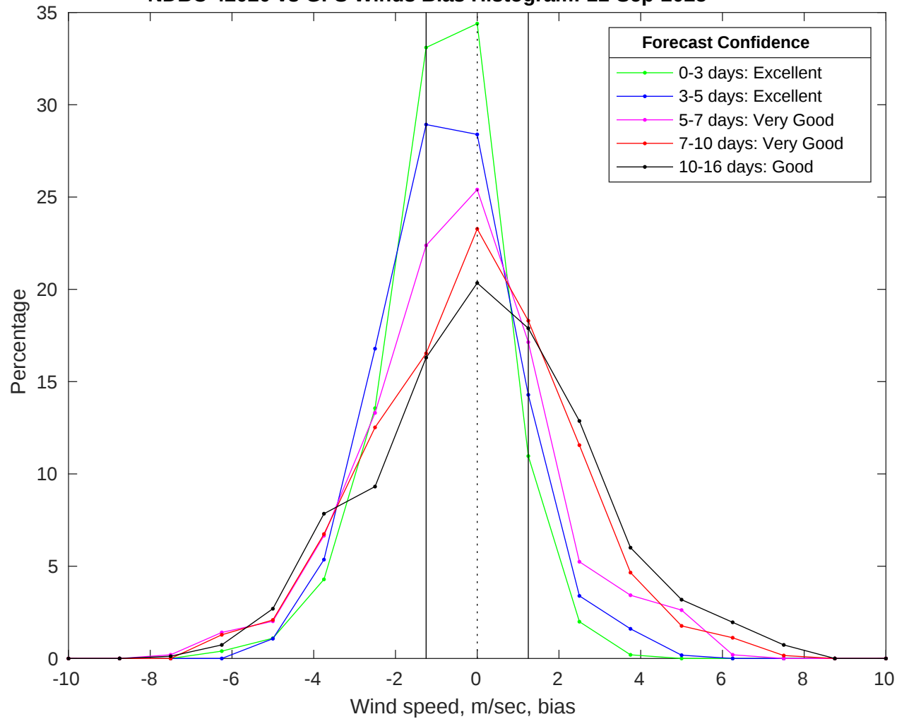
NDBC 42020 vs GFS Winds Bias Histogram: 11-Sep-2025
