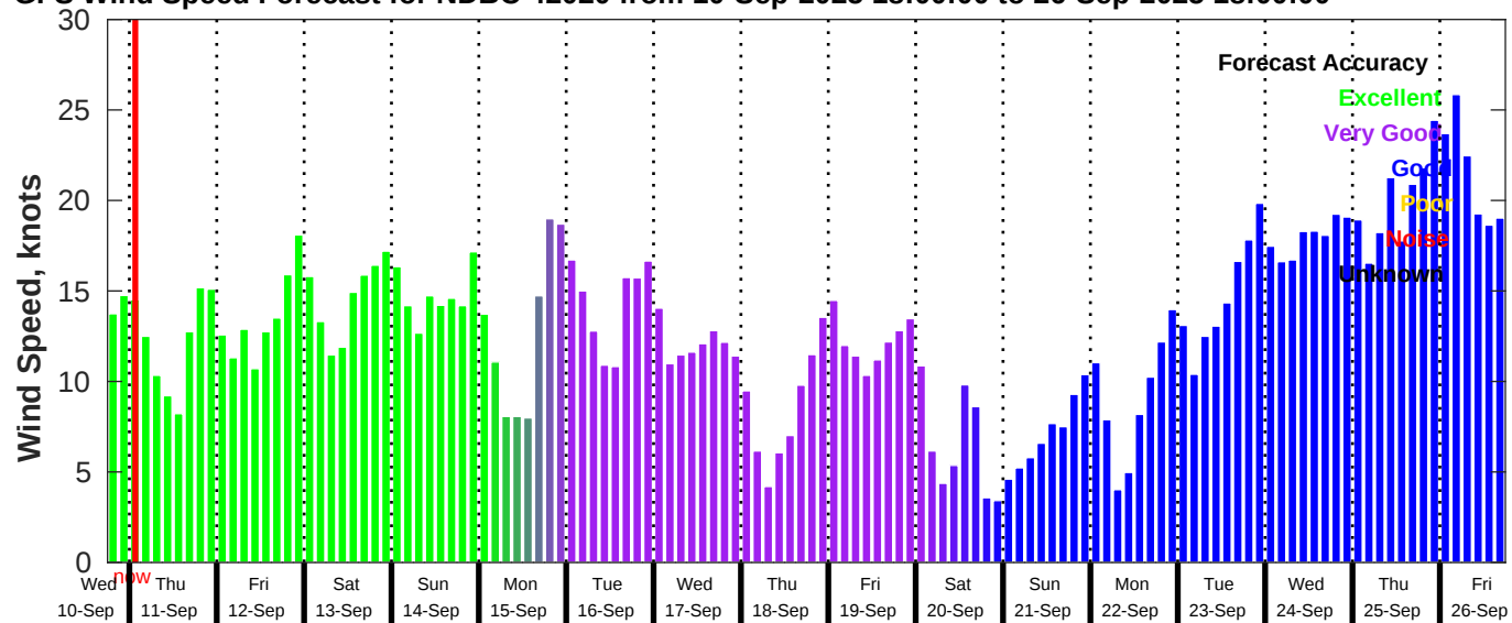
GFS Wind Speed Forecast for NDBC 42020 from 10-Sep-2025 18:00:00 to 26-Sep-2025 18:00:00
