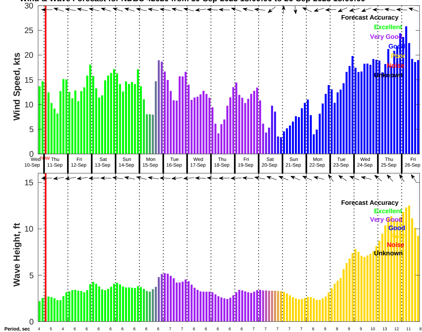
Wind & Wave Forecast for NDBC 42020 from 10-Sep-2025 18:00:00 to 26-Sep-2025 18:00:00
