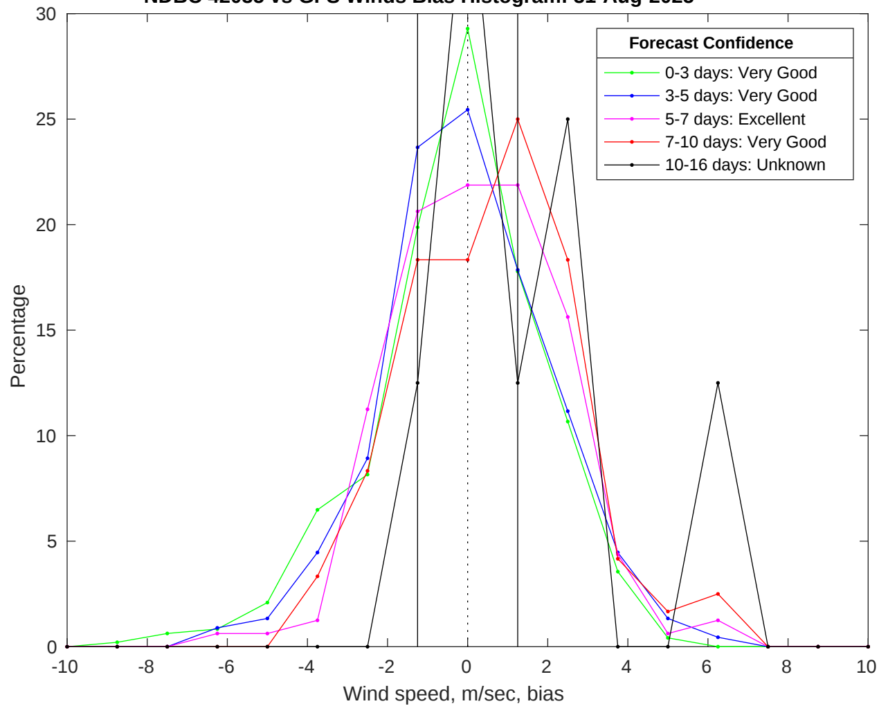
NDBC 42035 vs GFS Winds Bias Histogram: 31-Aug-2025
